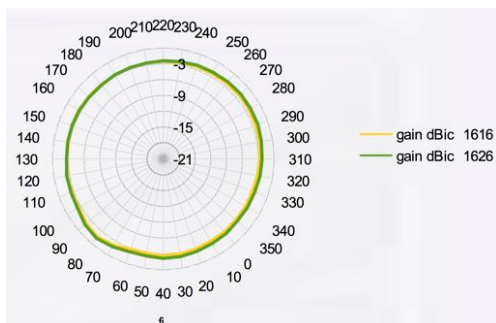
GAIN AZIMUTHAL
